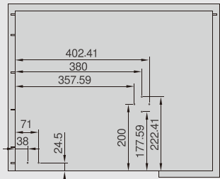
Bottom panel fixing holes
