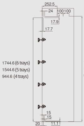
Screw positions of cabinet side left
