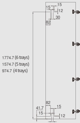
Screw positions of cabinet door
