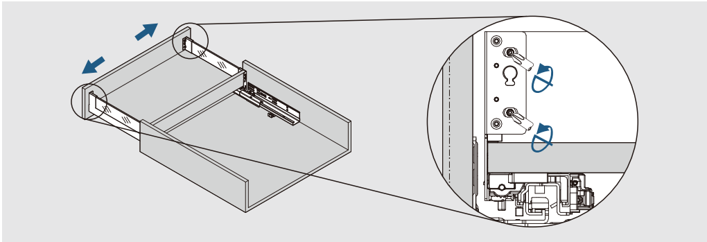
Left & right adjustment
