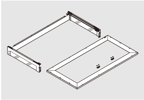
Bottom frame and brackets assembly
