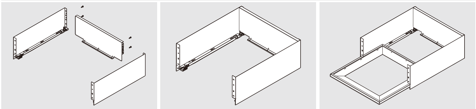
Metal back assembly Bottom frame assembly
