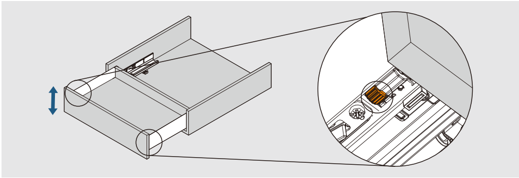
Up & down adjustment
