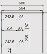
600mm wide cabinet: Bottom panel drilling
