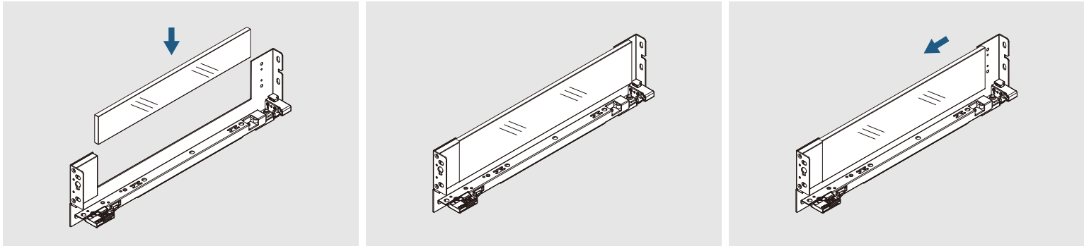
Insert glass-boxside
