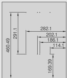
Front fixing holes
