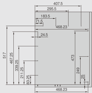
Left side panel fixing holes
