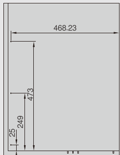
Right side panel fixing holes
