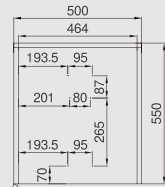
500mm wide cabinet: Bottom panel drilling
